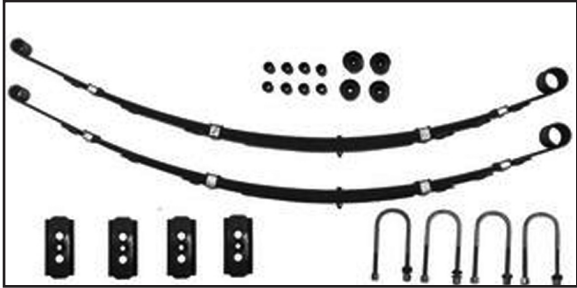
1959-1966 Rear Leaf Spring Kit
