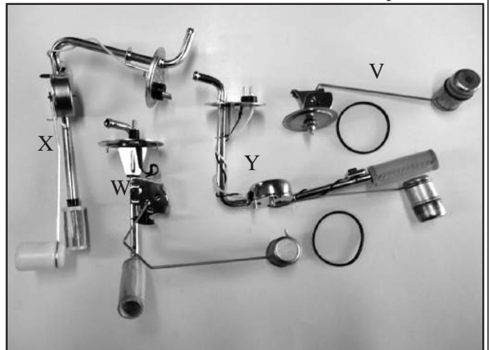
1964 - 1966 Fuel Tank
