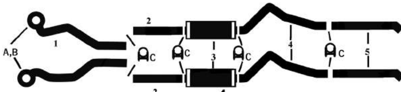
Typical muffler location for Extreme mufflers
